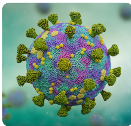
SARS-CoV-2 virus
